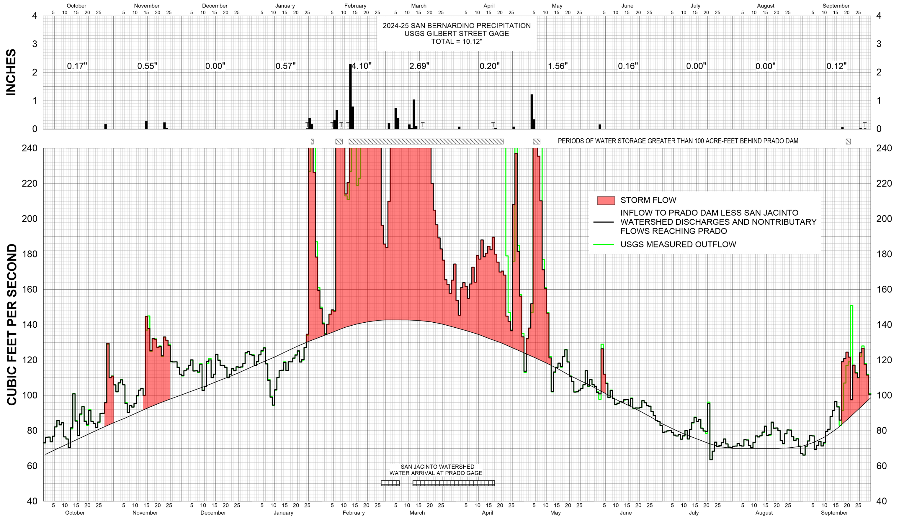
DISCHARGE OF THE SANTA ANA RIVER AT PRADO DAM & SAN BERNARDINO PRECIPITATION WATER YEAR 2024-25
