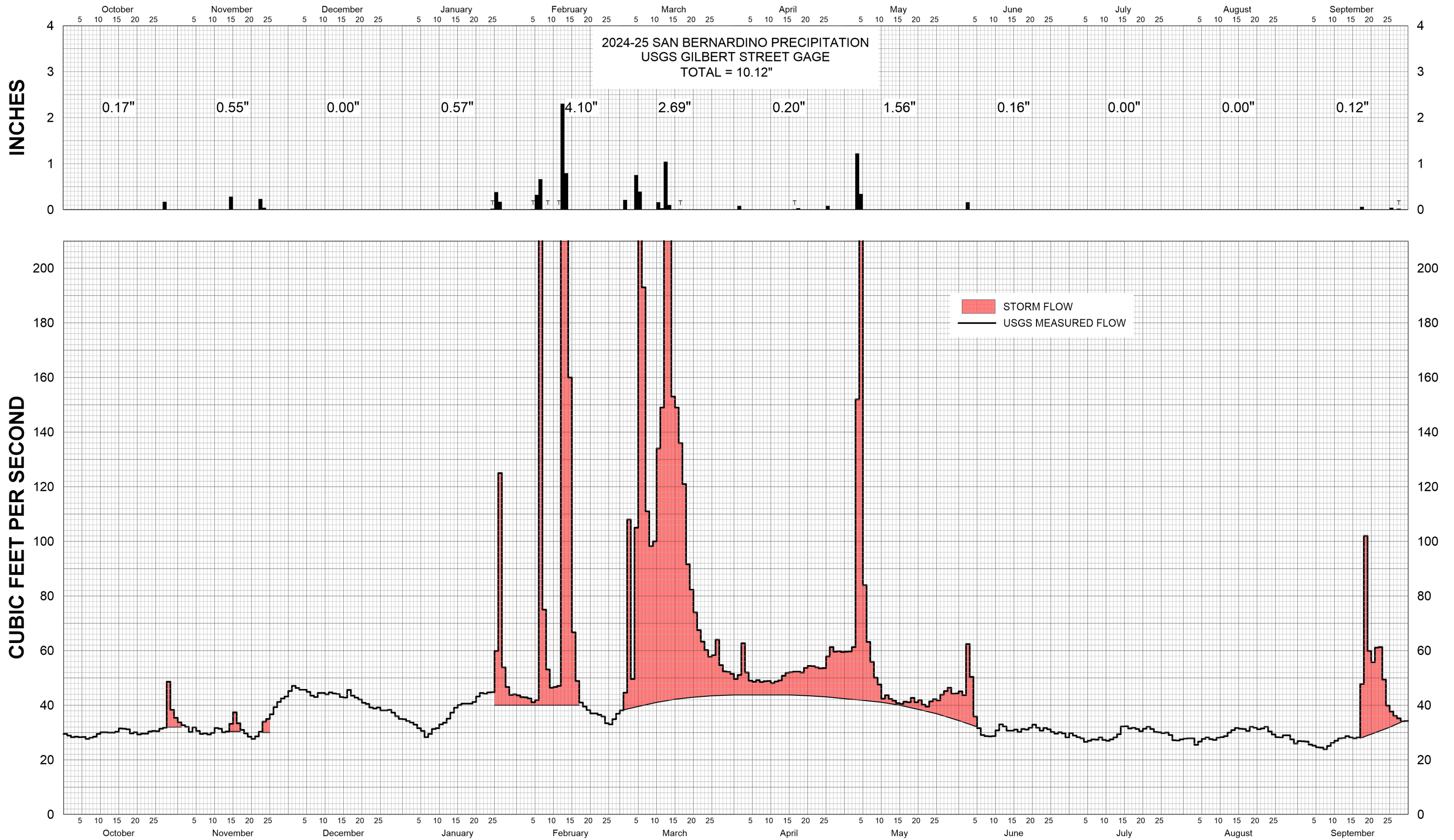
DISCHARGE OF SANTA ANA RIVER AT RIVERSIDE NARROWS & SAN BERNARDINO PRECIPITATION WATER YEAR 2024-25
