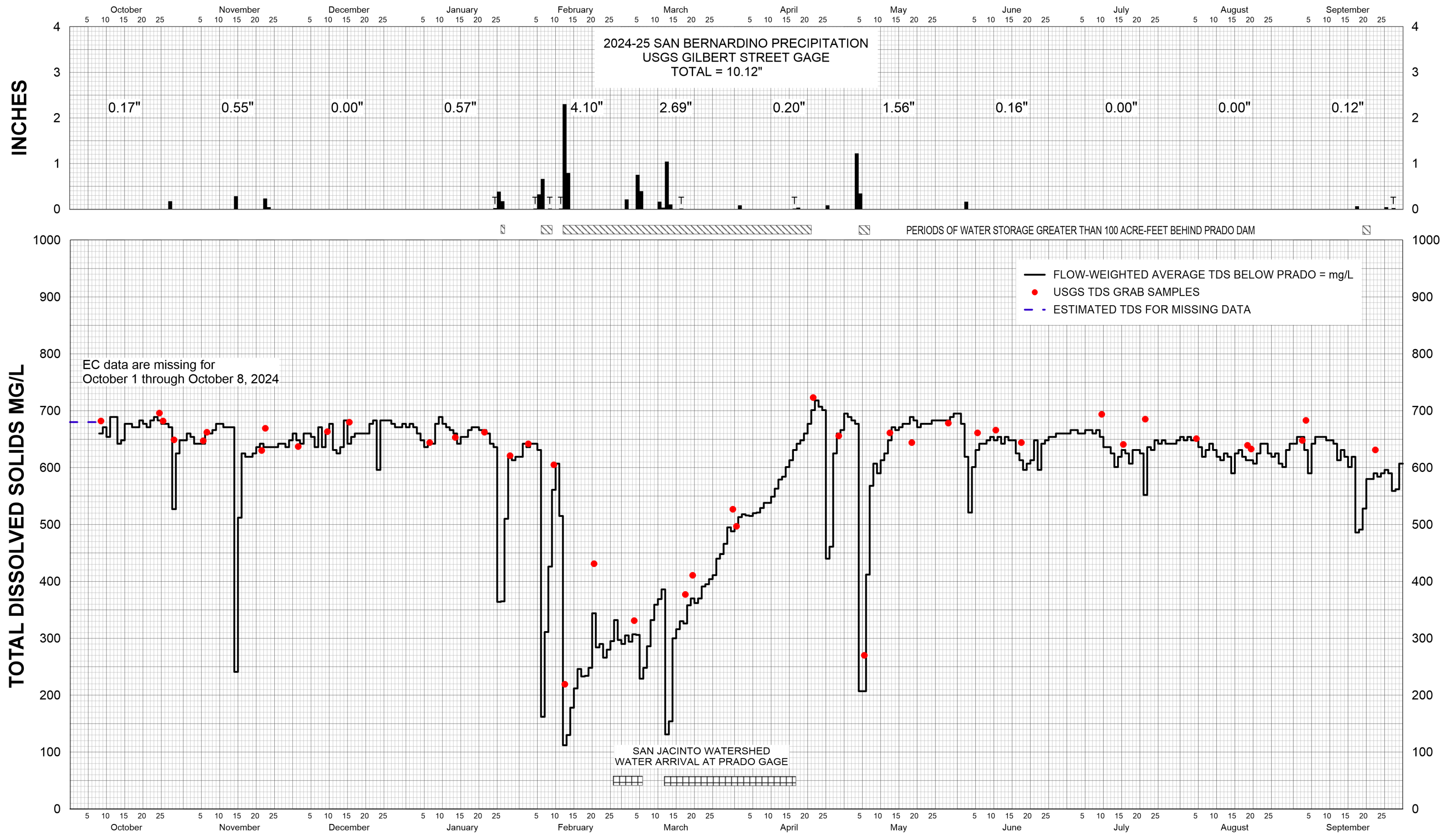
DISSOLVED SOLIDS IN SANTA ANA RIVER BELOW PRADO DAM WATER YEAR 2024-25
