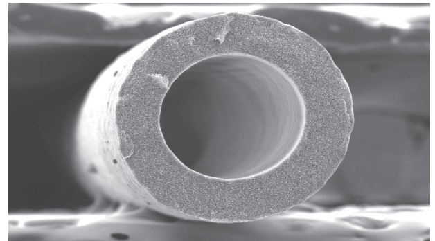
Microphotograph of a single microfiltration fiber. The GWRS contains 32,832 MF membranes, each housing approximately 15,000 fibers.
