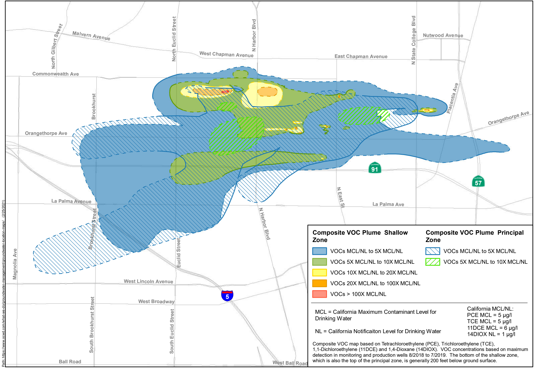
Composite North Basin VOC Plume Map (8/2018 - 7/2019) Plume map prepared by AECOM 1/2021
