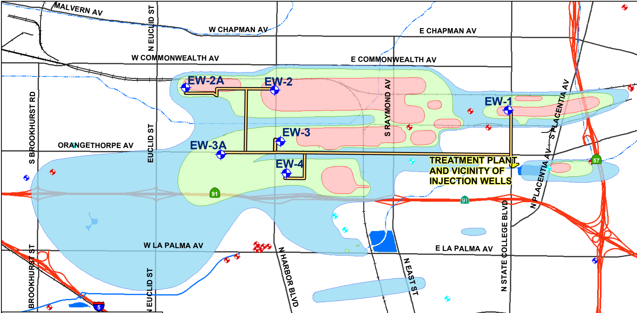
Composite VOC Plume Map (October 2008) and Containment System Layout (updated January 2009) NORTH BASIN GROUNDWATER PROTECTION PROJECT
